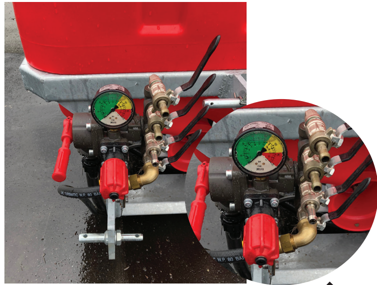
Spray Controller with Bypass Function. ↴
